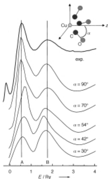
Figure 3. Comparison between experimental (top curve) and simulated XANES curves as a function of the angle \alpha of the \text{Cu}(\text{CO})_3 adduct in C_{3v} symmetry (1 Ry \approx 13.6 eV). Simulated spectra are calculated above the interstitial potential level only ( E > 0 ). Vertical lines indicate the position of bands A and B of the experimental spectrum. The schematic diagram represents the \text{Cu}^{\text{I}}(\text{CO})_3 adduct in C_{3v} symmetry and defines the angle \alpha .
